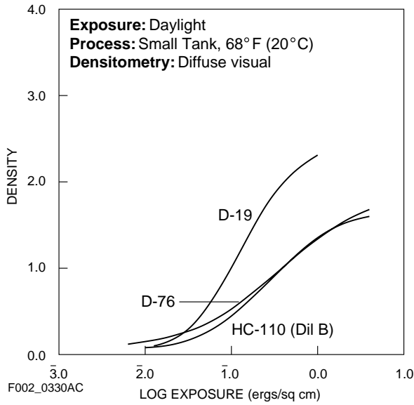
Characteristic Curves for KODAK High Speed Infrared Film / HIE
